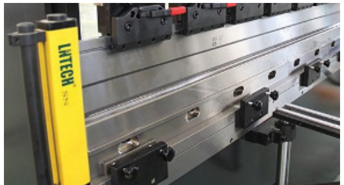
LHTECH Light Curtain Safety
