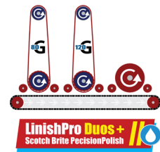
Twin Station Linisher With Polish Roller
